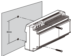
Mounting method 1: Direct mounting. use two screws to fix the VD 2KR on the wall Directly
