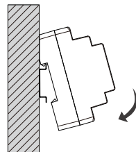
Mounting method 2: DIN nail mounting. Slot the VD 2KR on the DIN nail.
